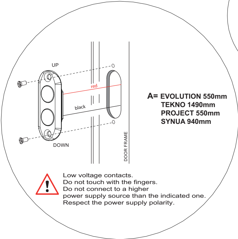
Connection on the door with a corrugated sheath. Use a cable with 2x1mm section, featuring a max. distance of 20m between the lock and power supply unit.
