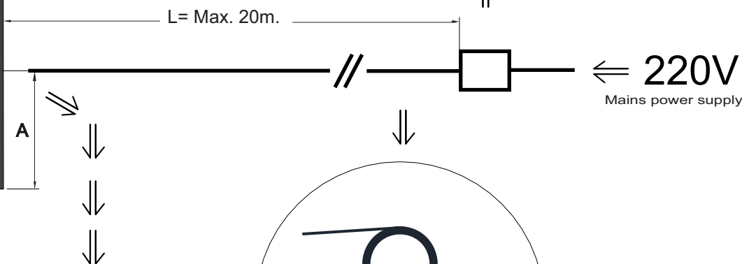
Connection on the door with a corrugated sheath. Use a cable with 2x1mm section, featuring a max. distance of 20m between the lock and power supply unit.
